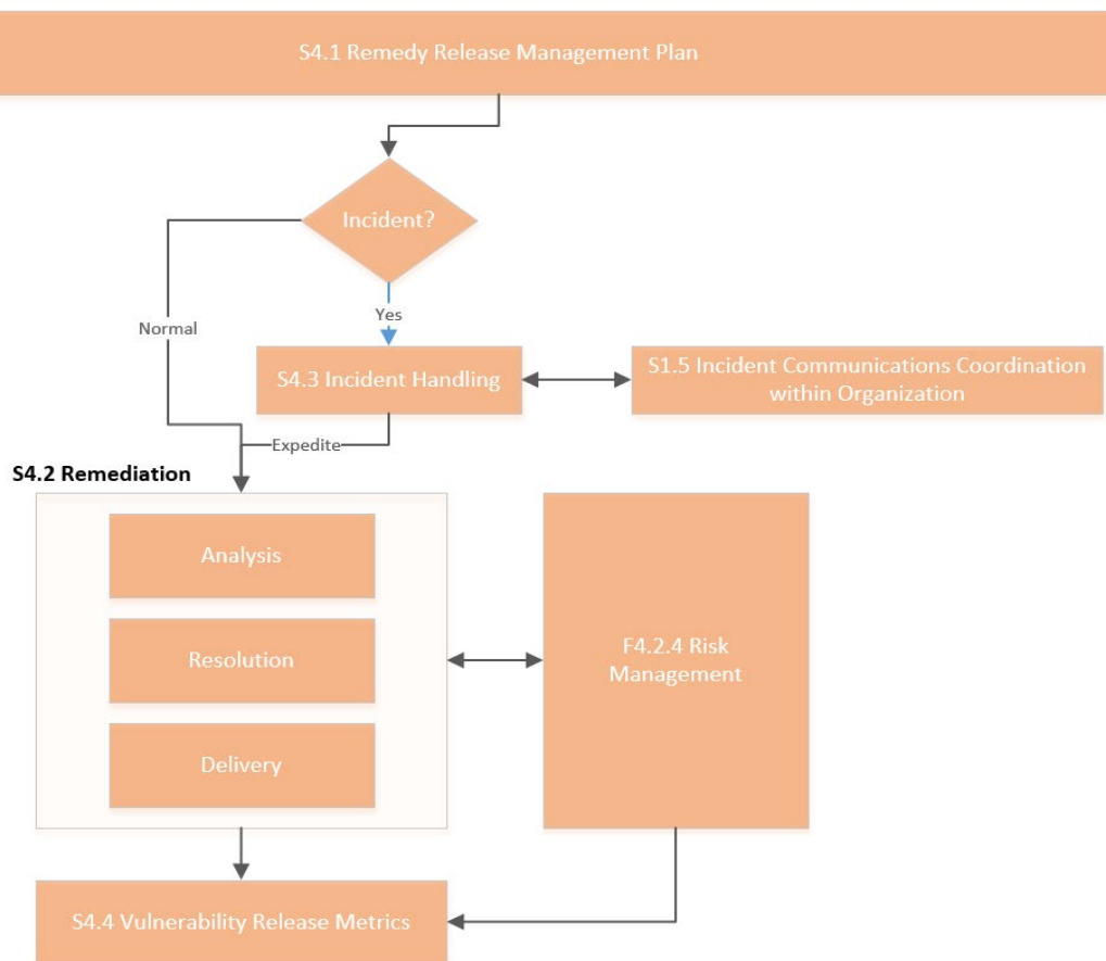
Figure 11: Ex. of a Core Remedy Release Process
